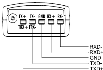
RS485
